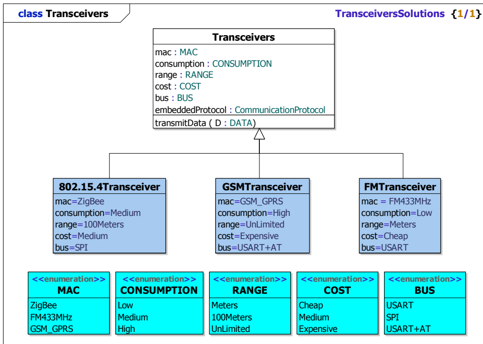
Fig. 10. Details of transceiver diagram
