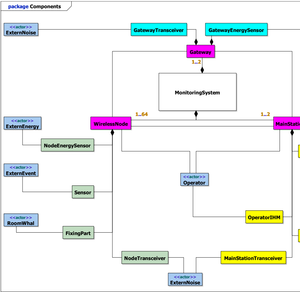
Fig. 4. Initial class diagram
