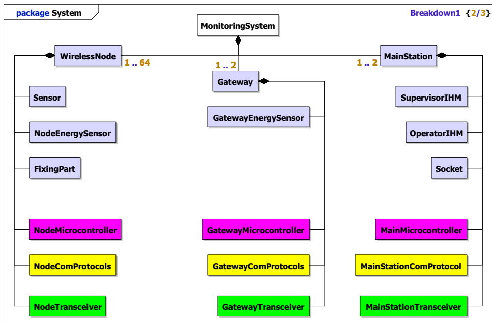
Fig. 8. Microcontrollers and protocols components
