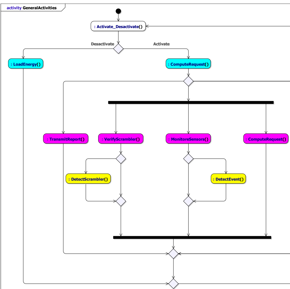
Fig. 6. General activity diagram
