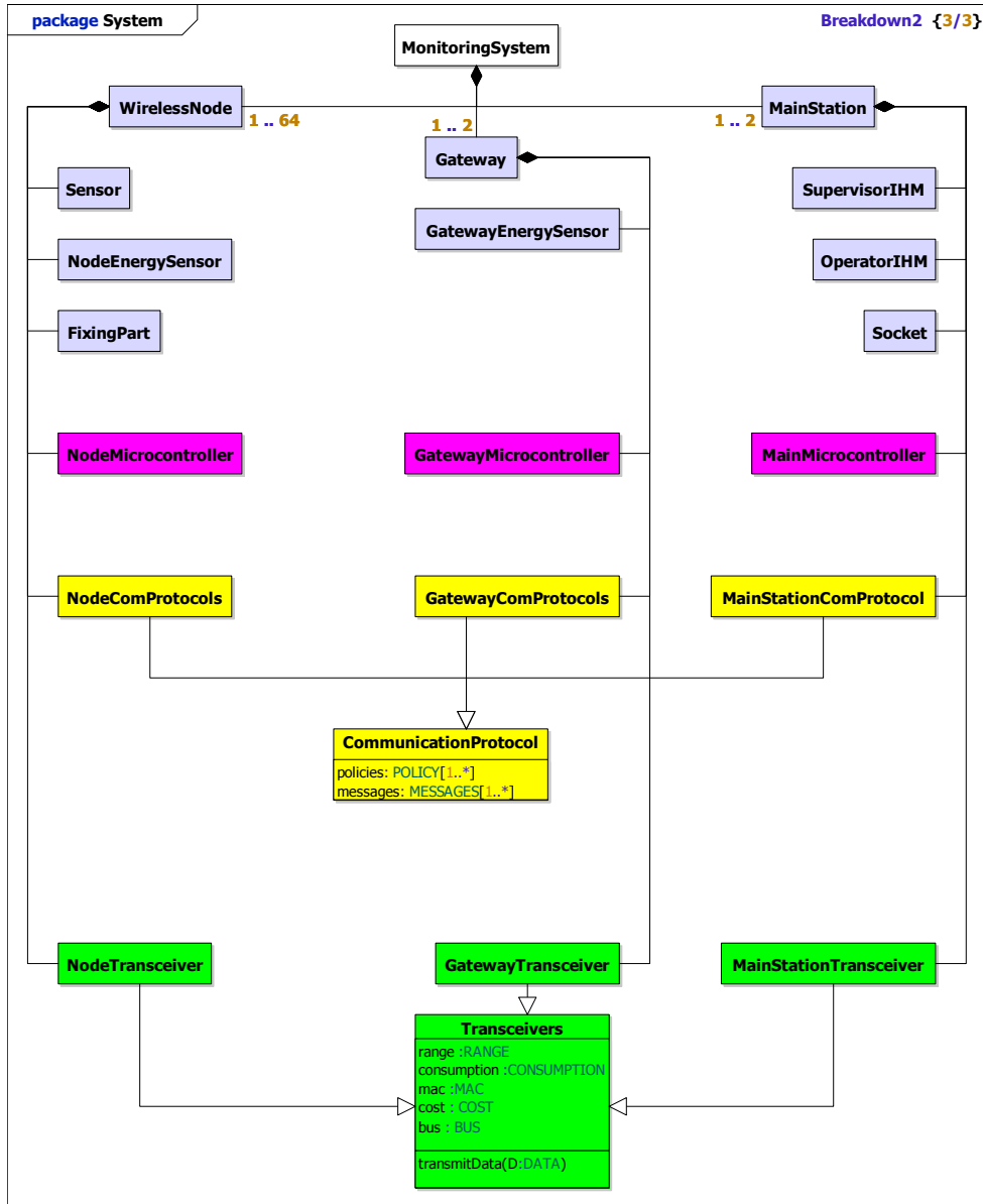
Fig. 9. Final class diagram
