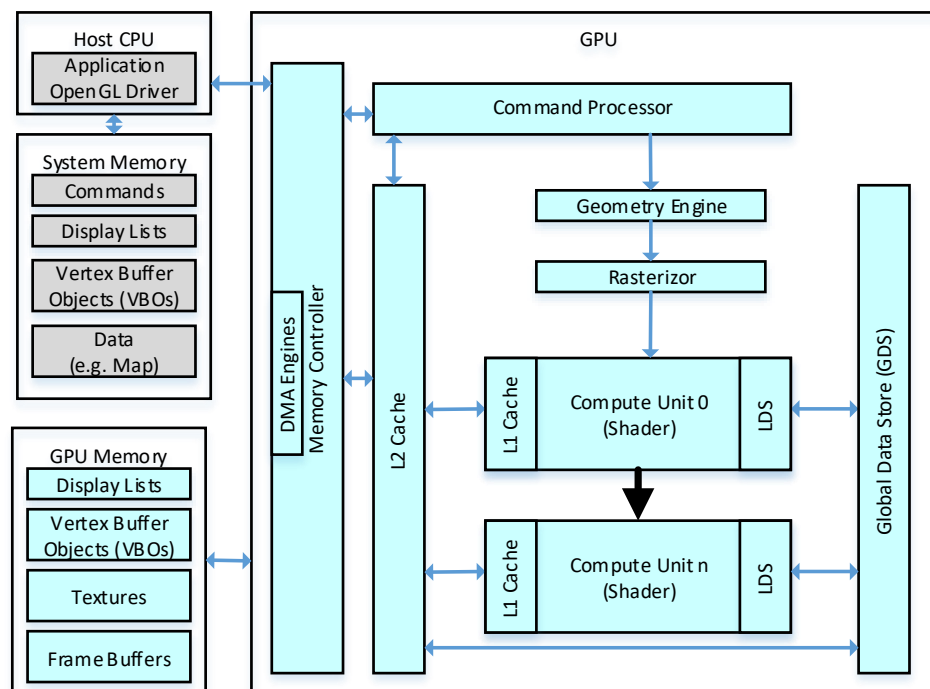
Figure 1: General GPU High Level Architecture Diagram
