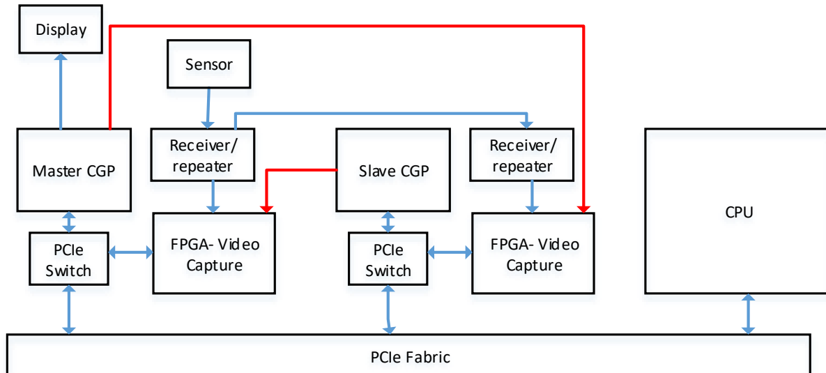
Figure 13: Redundant CGP with Cross-Monitoring.
